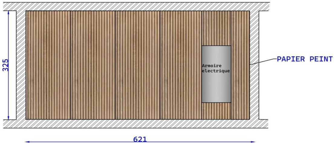
Detail Mur B
